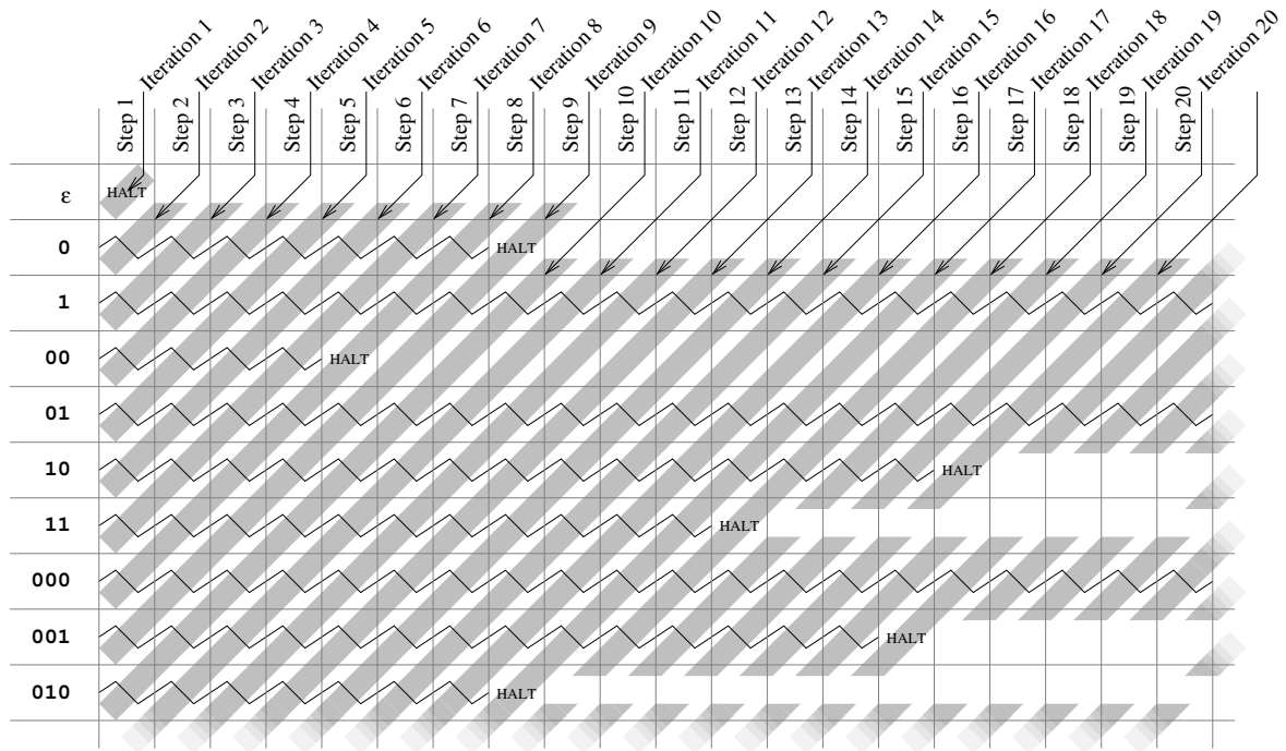
Figure 1.2: Enumerating all halting machines (on empty tape): top: the algorithm; bottom: a working schematic
