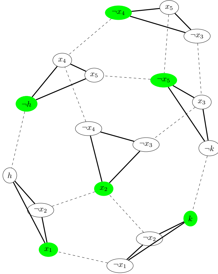
Figure 3.1: Reduction of the 3-CNF formula (3.8) to a graph for INDSET.
