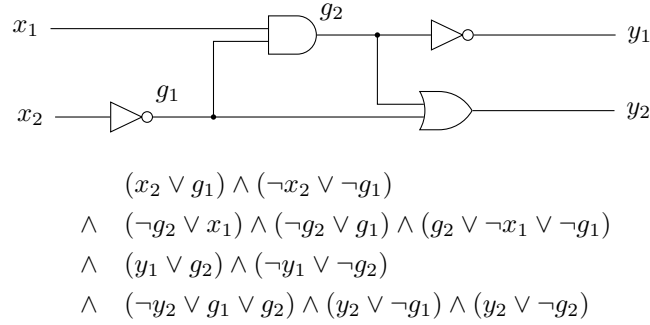
Figure 3.4: A Boolean circuit and its 3-CNF representation: the 3-CNF formula is satisfiable by precisely the combinations of truth values that are compatible with the logic gates.
