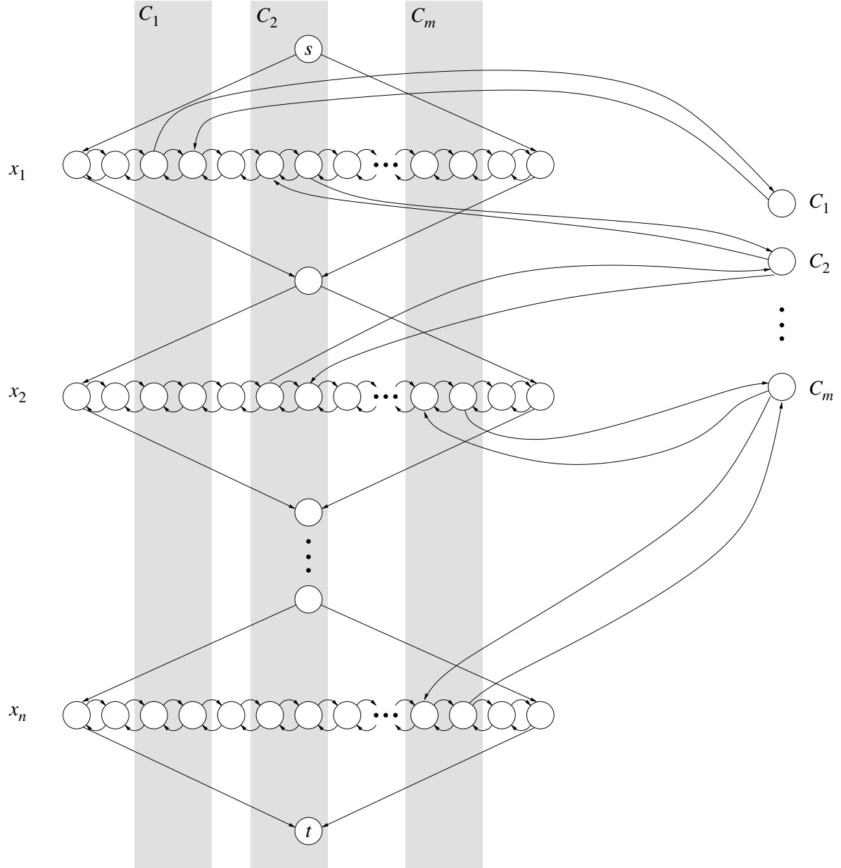
Figure 3.11: Representation of formula (x_1 \vee \dots) \wedge (\neg x_1 \vee x_2 \vee \dots) \wedge \dots \wedge (\neg x_2 \vee \dots \vee x_n) .
