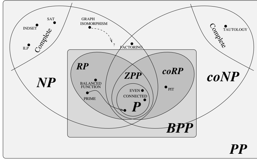
Figure 5.5: What we know about the probabilistic classes introduced in this Section. In particular, the relationship between BPP and NP is unknown.
