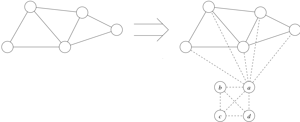
Figure 5.4: Reducing a 3-VERTEX COLORING instance to an equivalent 4-VERTEX COLORING instance.
