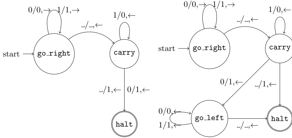
Figure 5.3: A non-oblivious TM (left) and an equivalent oblivious version (right).
