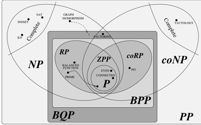
Figure 5.6: Position of the BQP quantum class in the previous diagram, with the notable inclusion of the FACTORING language.
