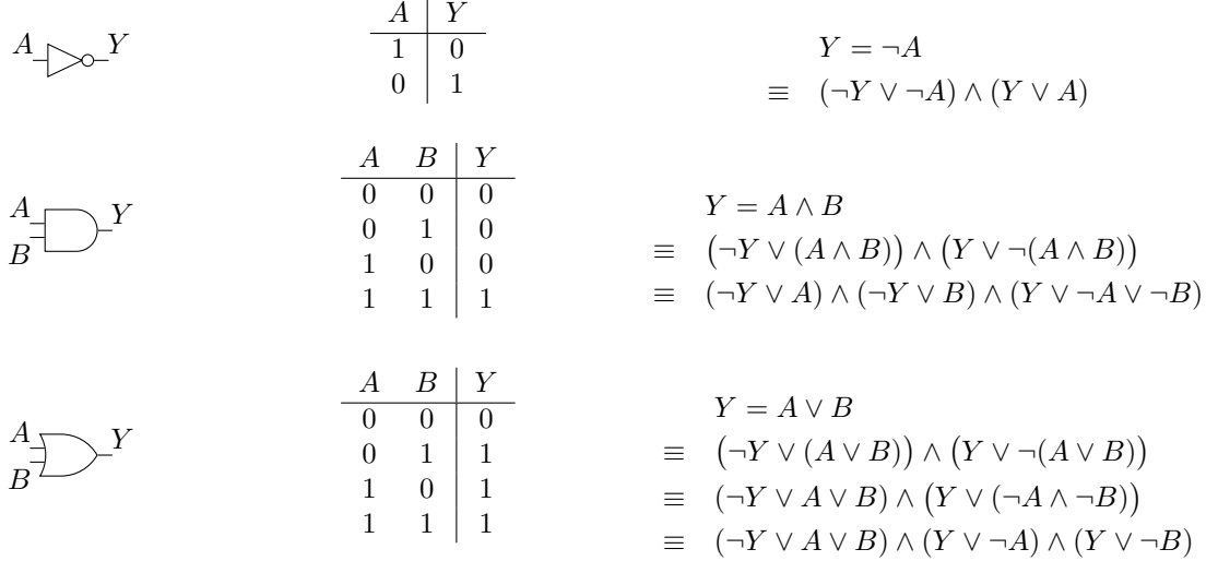
Figure 3.3: A NOT gate (top), an AND gate (middle) and an OR gate (bottom), their truth tables, and derivations of the 3-CNF formulas that are satisfied if and only if their variables are in the correct relation (i.e., only by combinations of truth values shown in the corresponding table).
