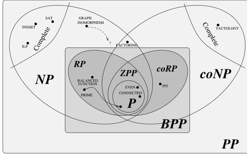
Figure 6.4: What we know about the probabilistic classes introduced in this Section. In particular, the relationship between BPP and NP is unknown.
