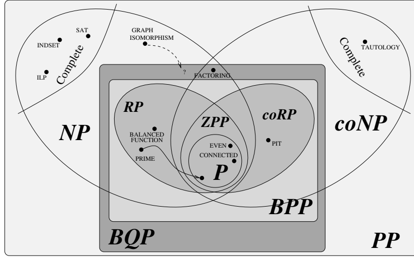
Figure 6.5: Position of the BQP quantum class in the previous diagram, with the notable inclusion of the FACTORING language.
