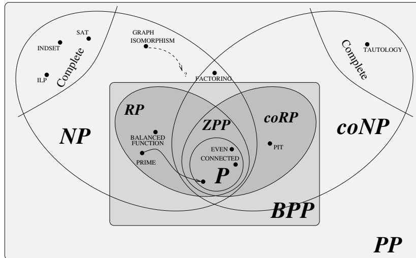
Figure 6.3: What we know about the probabilistic classes introduced in this Section. In particular, the relationship between BPP and NP is unknown.
